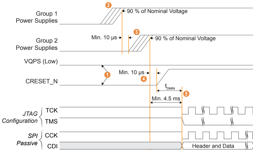
图 46: Power-Up Sequence
