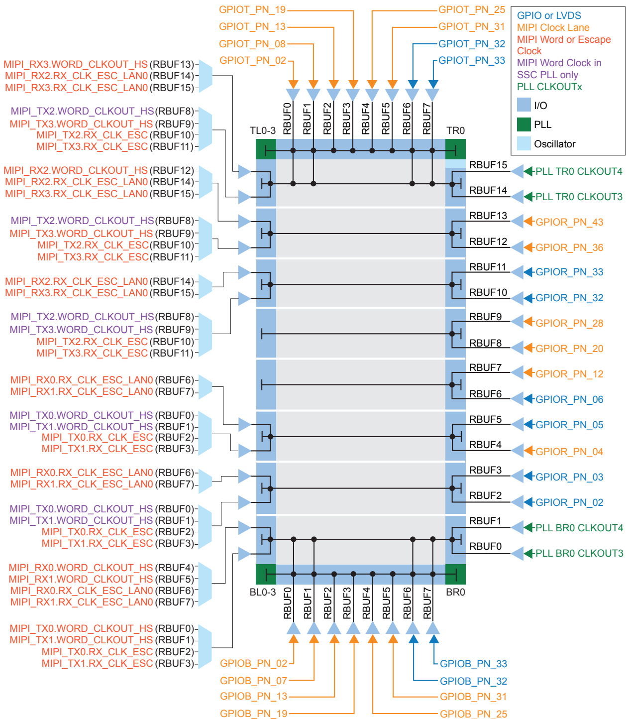
图 12: Clock Sources that Drive the Regional Network
