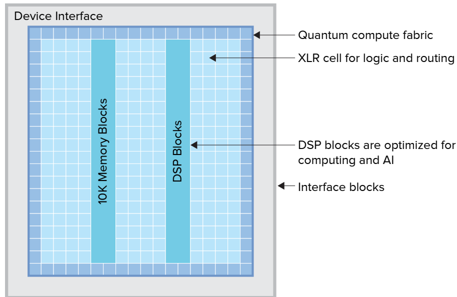
Fig 1: Ti180 FPGA Block Diagram
