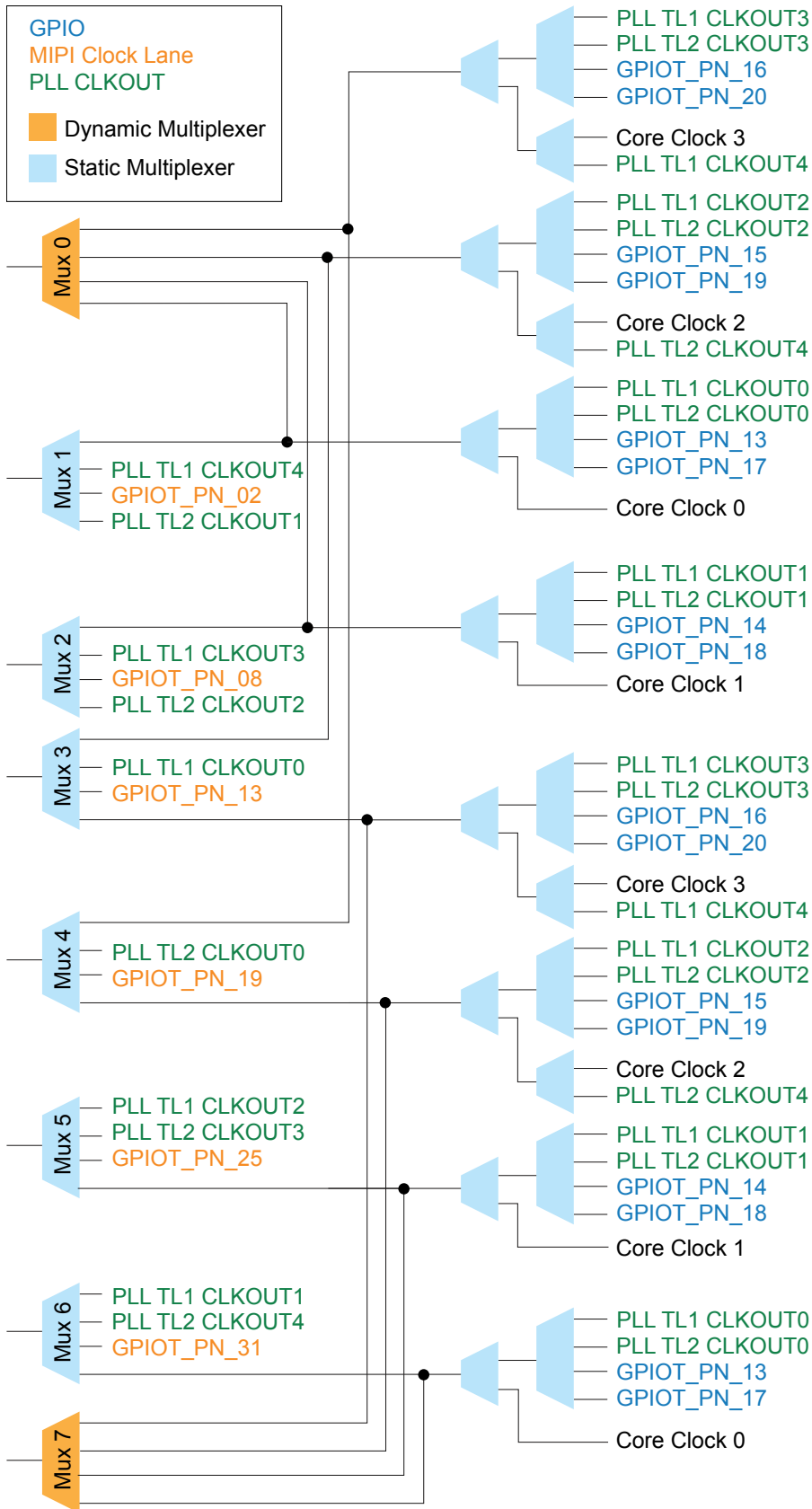
8: Clock Sources that Drive the Multiplexers: Top
