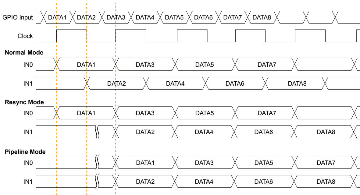
图 16: DDIO Input Timing Waveform
