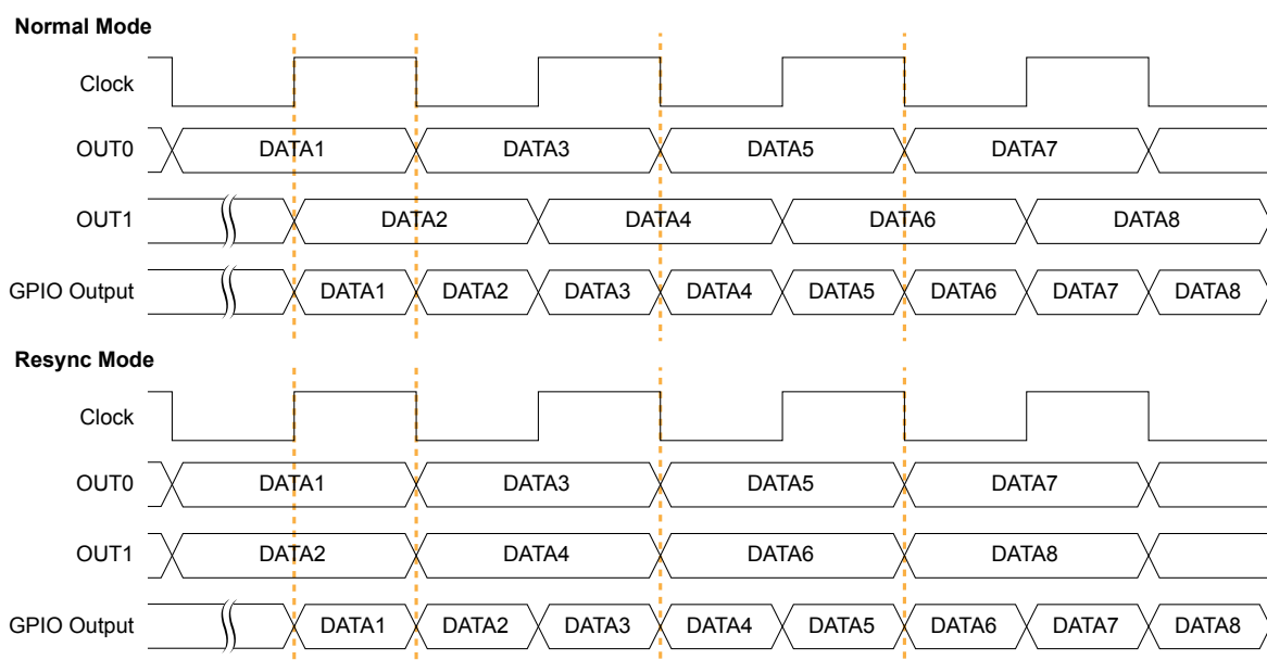
图 17: DDIO Output Timing Waveform
