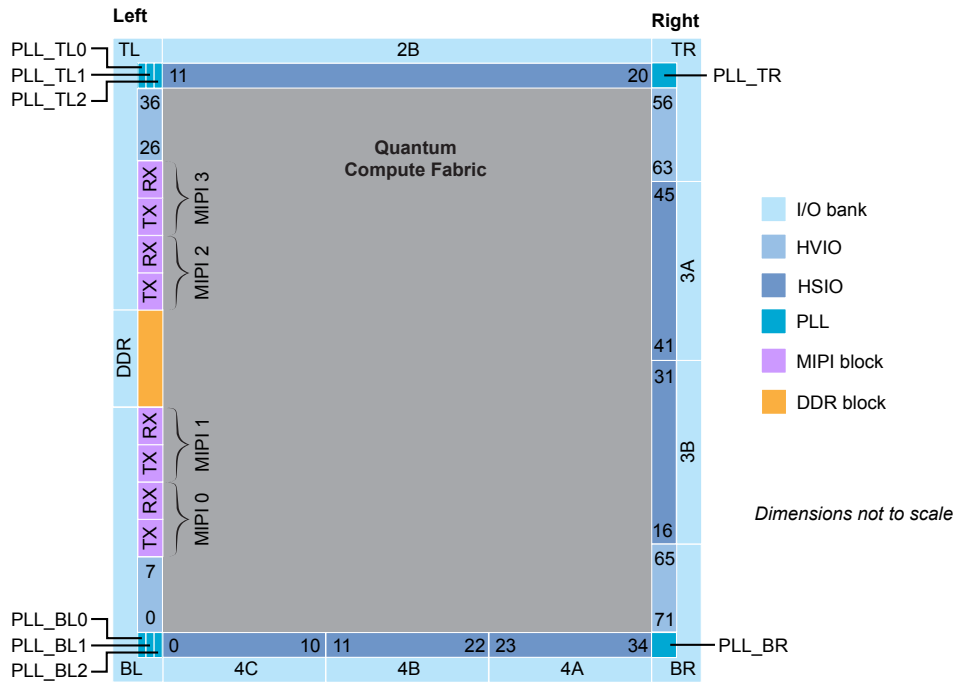
图 55: Floorplan Diagram for J484 and M484 Packages
