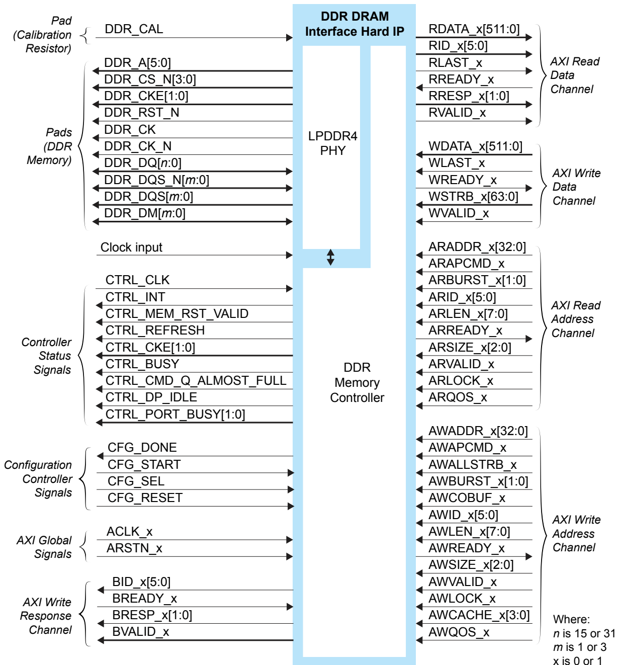
图 32: DDR DRAM Block Diagram
