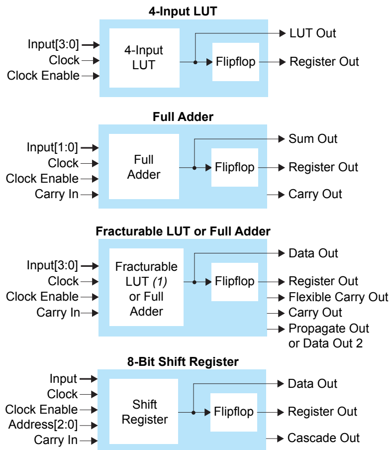
图 2: Logic Cell Functions
