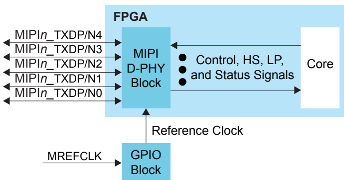
图 37: MIPI TX D-PHY Interface Block Diagram
