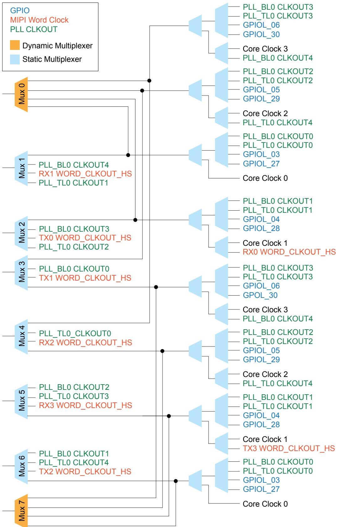
FIG 10: Clock Sources that Drive the Multiplexers: Left
