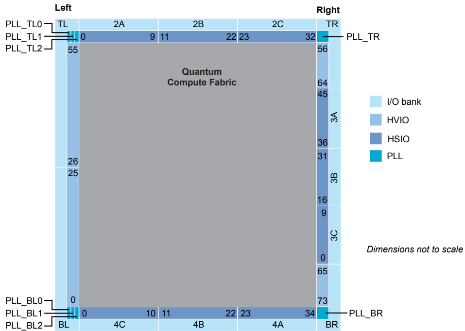
图 54: Floorplan Diagram for L484 Packages
