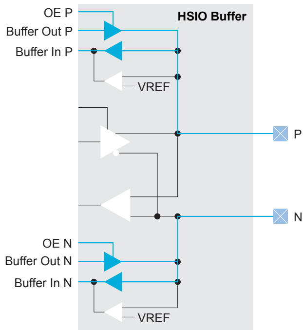
图 21: I/O Buffer Path for LVCMOS
