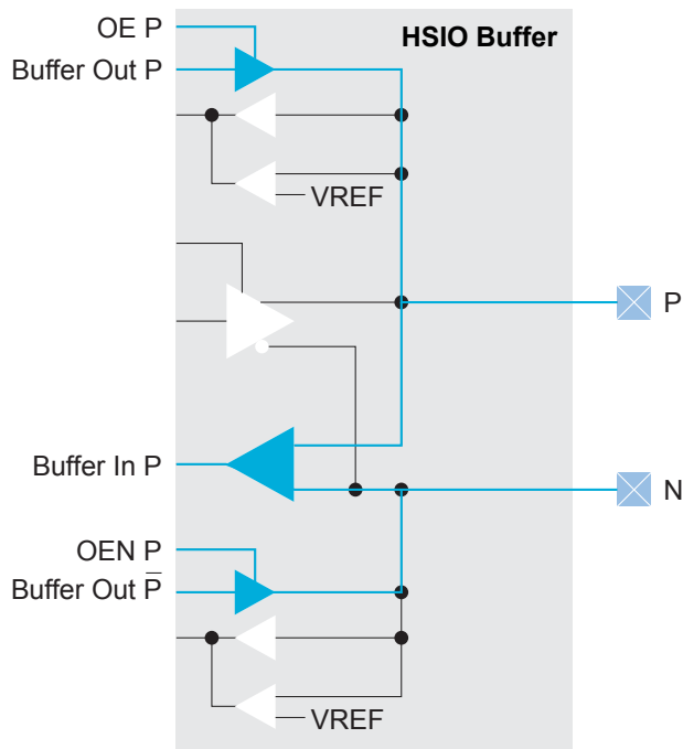
图 23: I/O Buffer Path for Differential HSTL and SSTL
