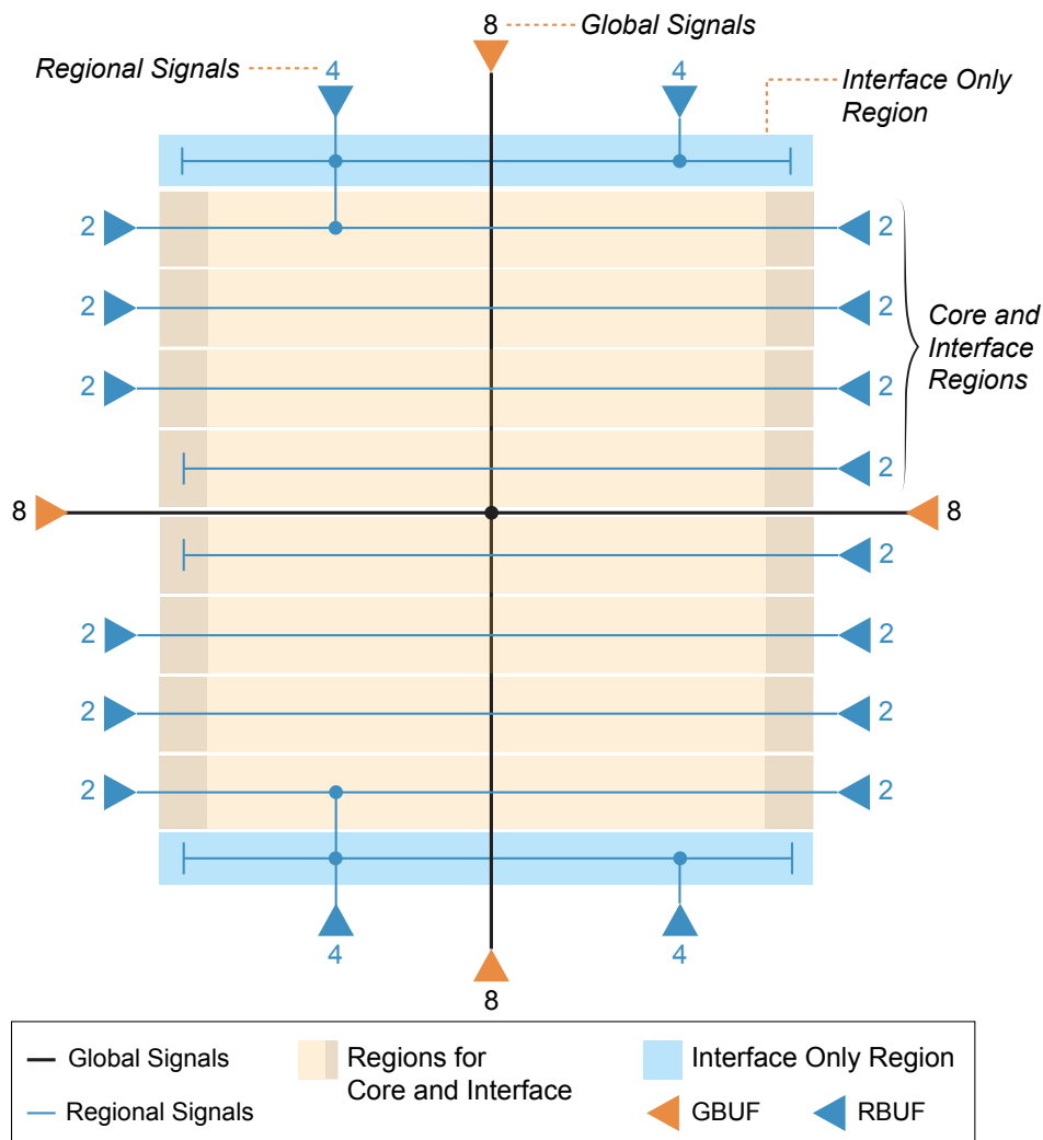
图 6: Global and Regional Clock Network Overview
