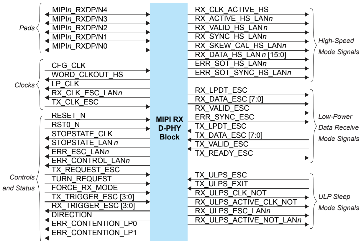
图 34: MIPI RX D-PHY x4 Block Diagram
