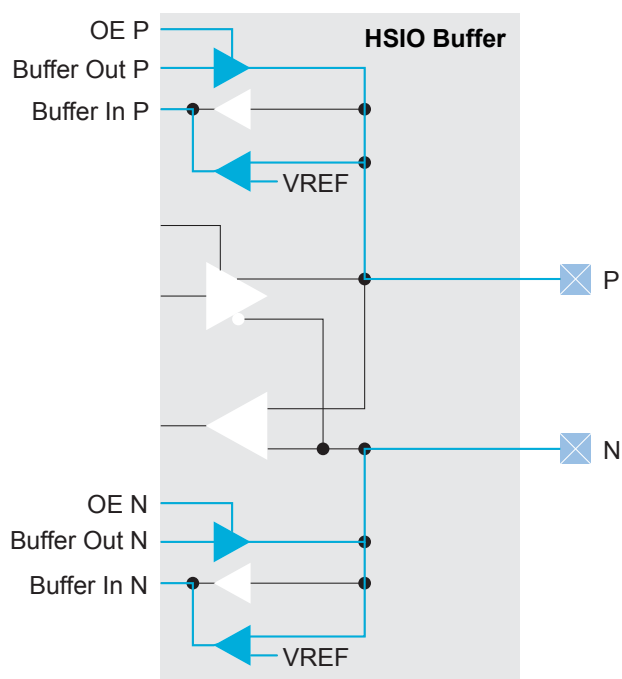
图 22: I/O Buffer Path for HSTL and SSTL
