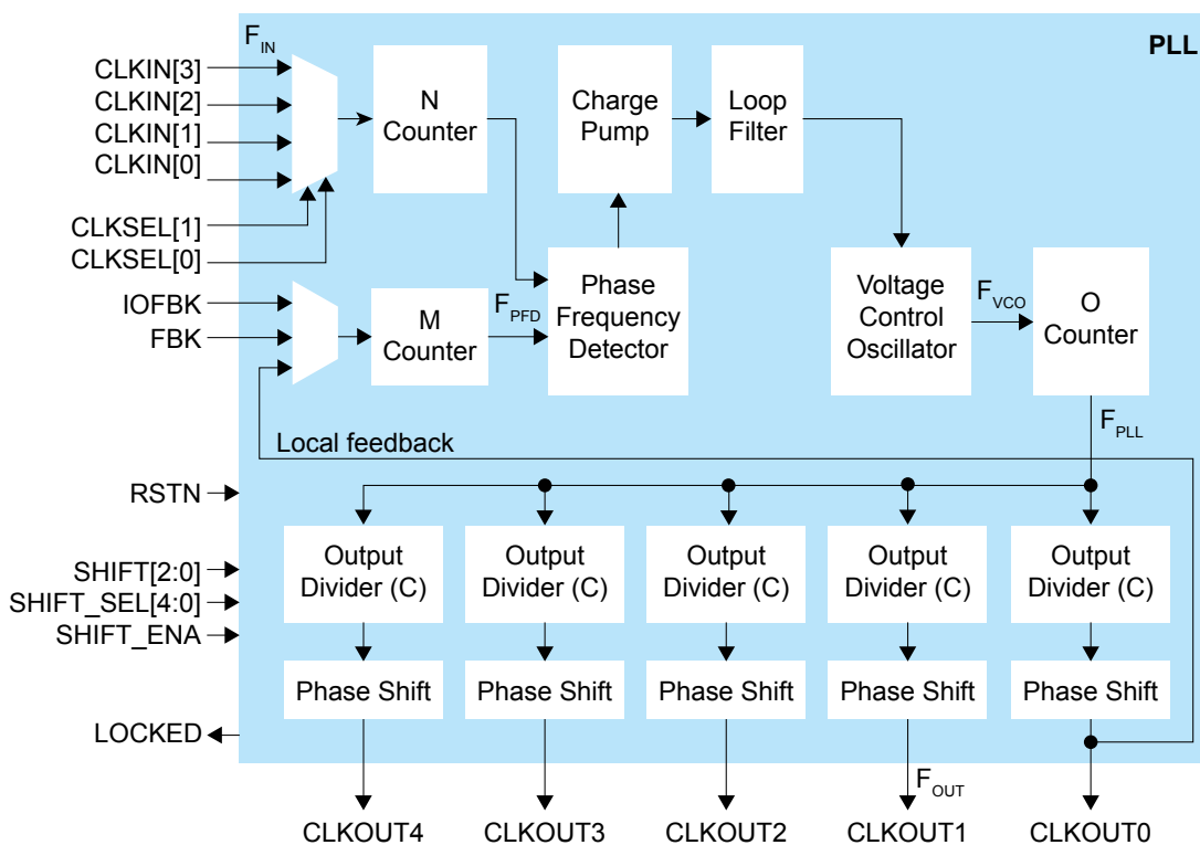
图 38: PLL Block Diagram
