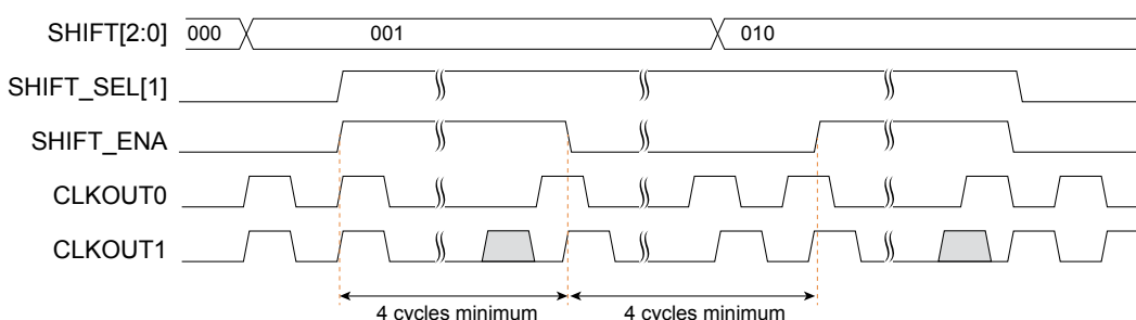
图 41: Consecutive Dynamic Phase Shift Waveform Example for CLKOUT1
