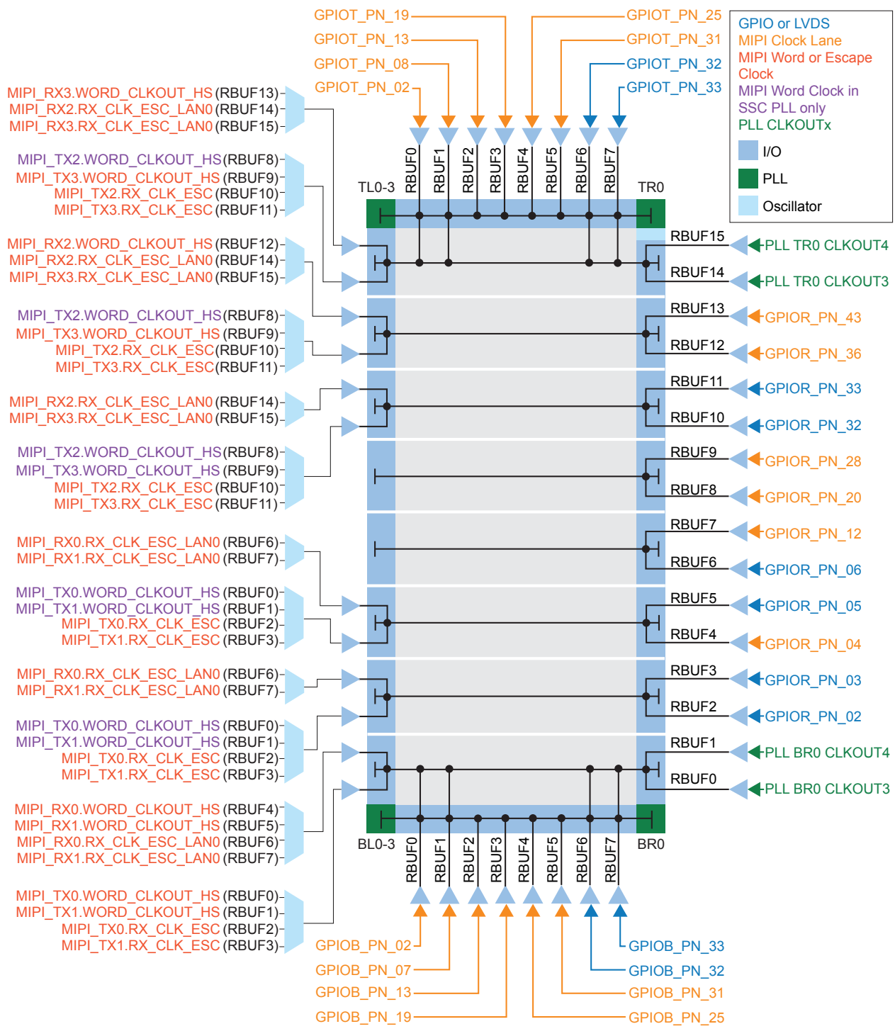
图 12: Clock Sources that Drive the Regional Network
