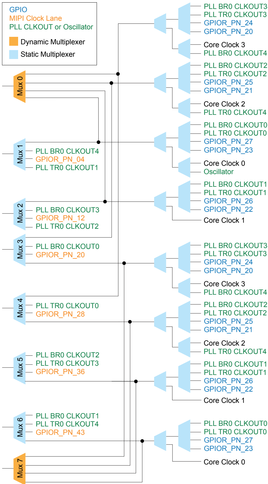
FIG 11: Clock Sources that Drive the Multiplexers: Right
