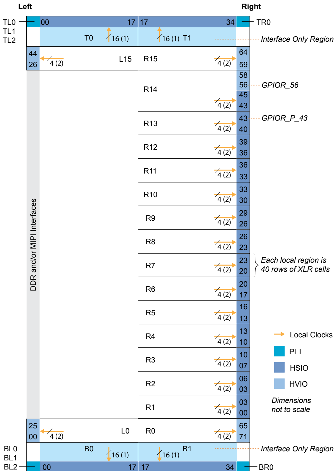
图 14: Clock Sources that Drive the Interfaces
