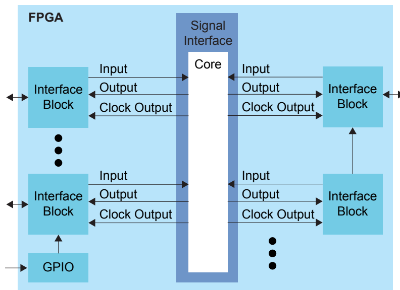
图 15: Interface Block and Core Connectivity
