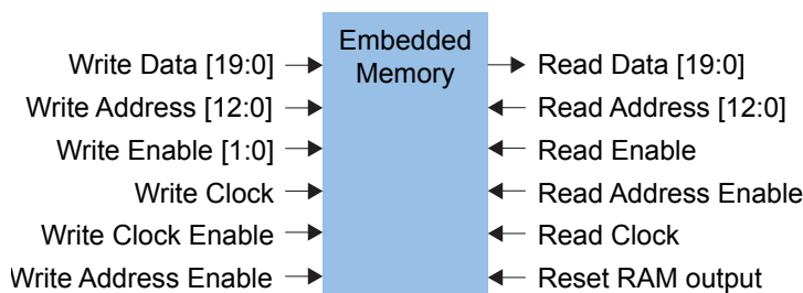
图 4: Simple Dual-Port Mode RAM Block Diagram (512 x 20 Configuration)
