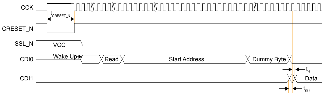
图 50: SPI Active (x1) Timing Sequence
