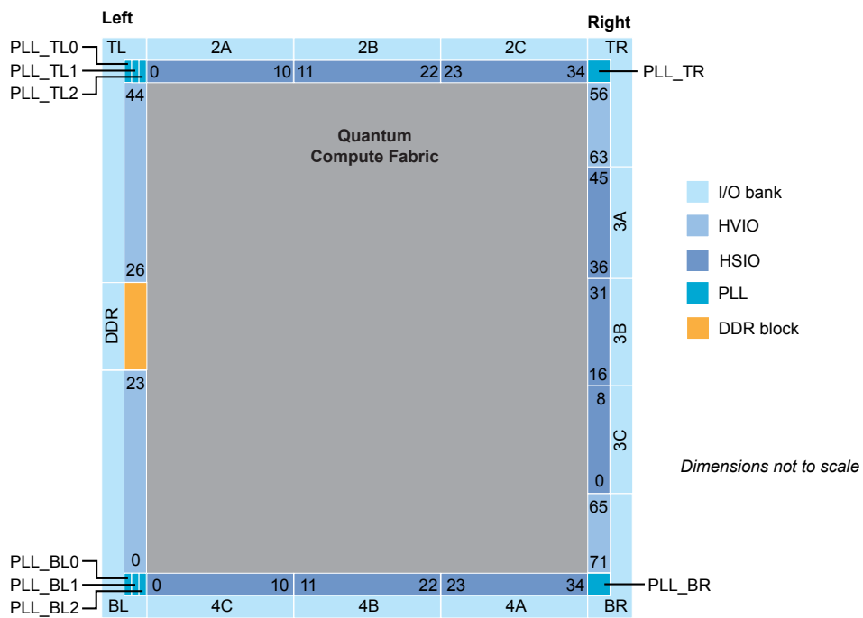
图 56: Floorplan Diagram for G529 Packages
