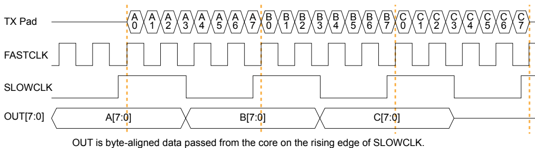
图 27: LVDS Timing Example Serialization Width of 8 (Half Rate)
