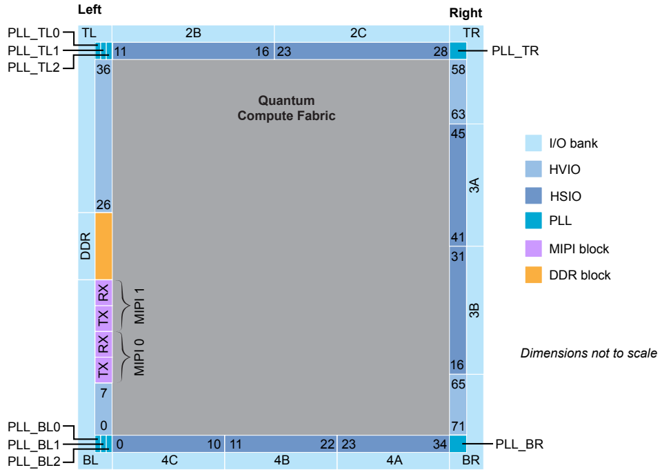
图 52: Floorplan Diagram for J361 Packages
