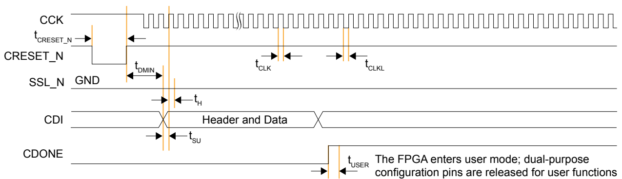
图 51: SPI Passive Mode (x1, Mode 3) Timing Sequence
