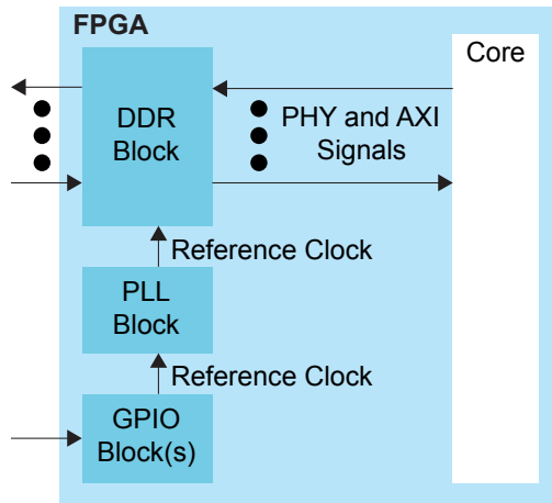
图 33: DDR DRAM Interface Block Diagram
