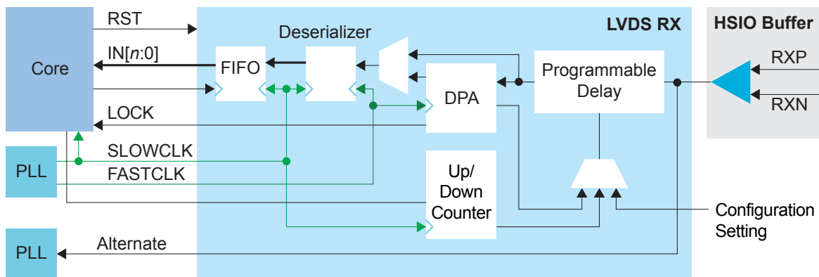
图 24: LVDS RX Interface Block Diagram
