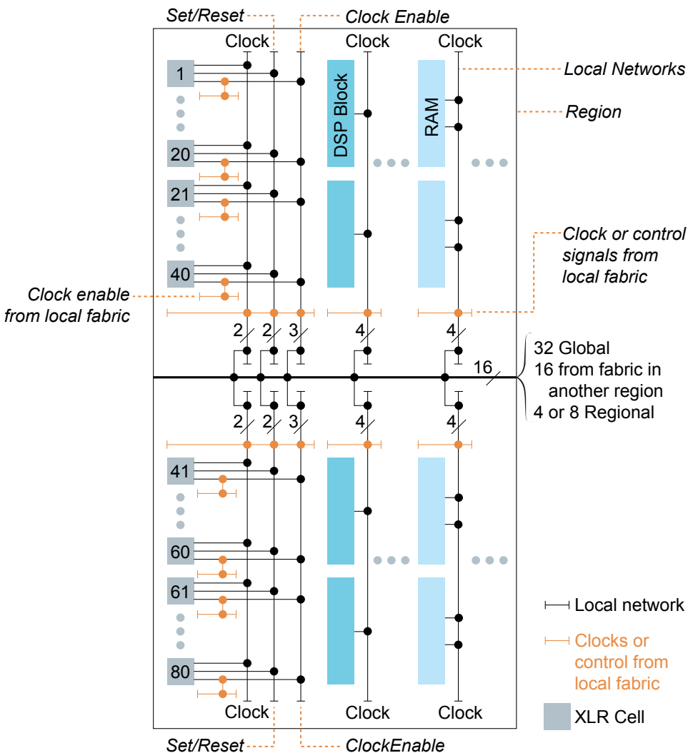
图 13: Clock Sources for Logic, DSP Blocks, and RAM
