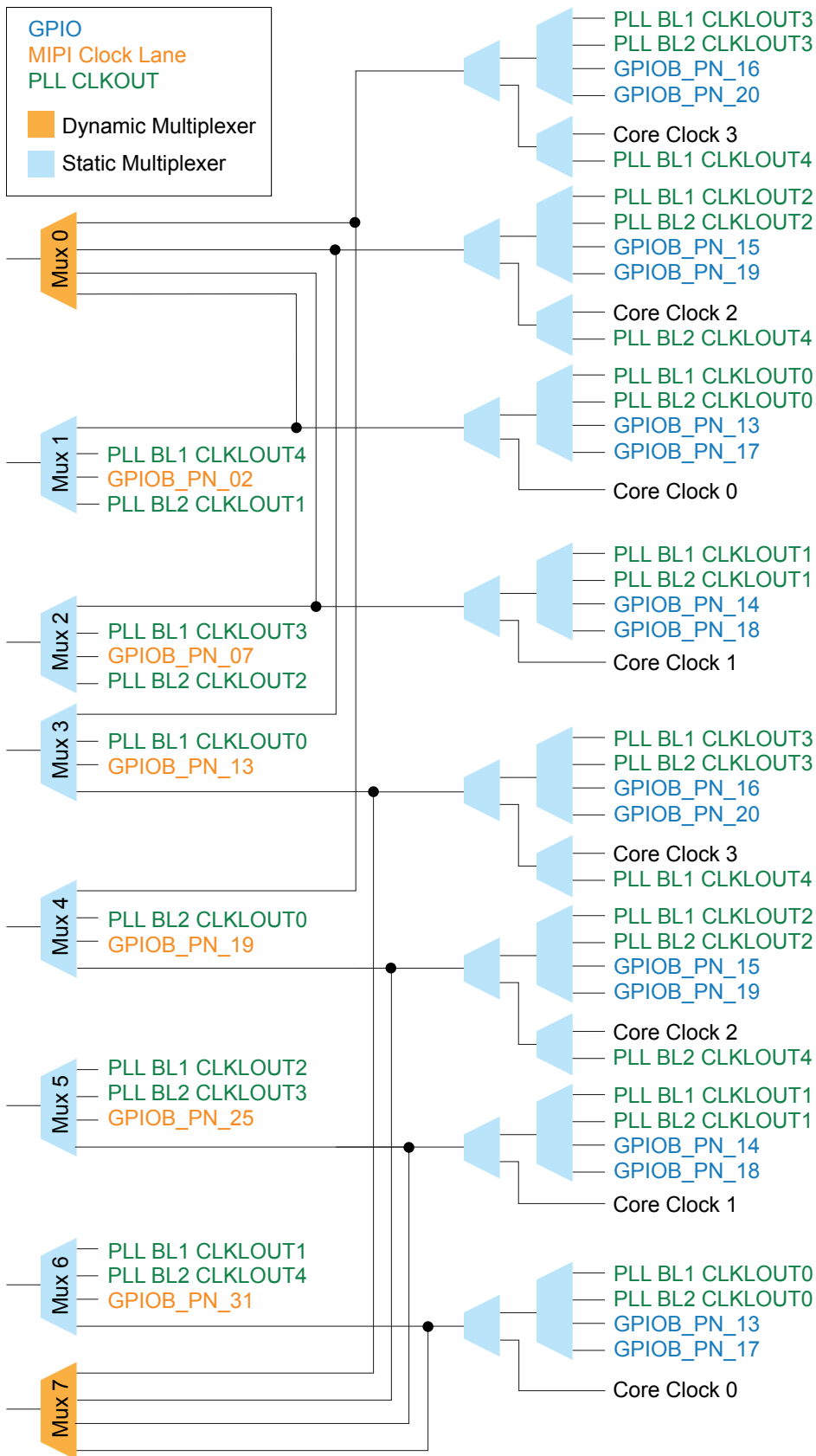
Fig 9: Clock Sources that Drive the Multiplexers: Bottom
