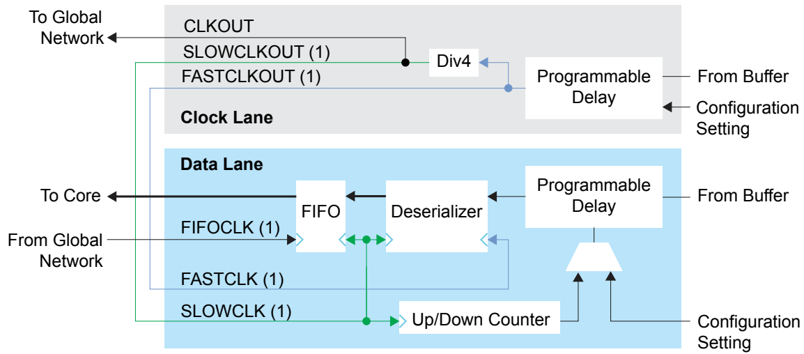
图 30: Connections for Clock and RX Data Lane in the Same MIPI RX Channel
