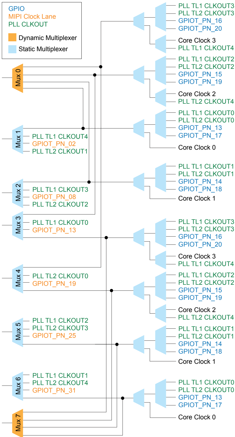
8: Clock Sources that Drive the Multiplexers: Top
