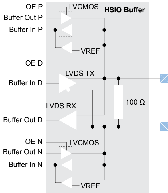
图 19: HSIO Buffer Block Diagram
