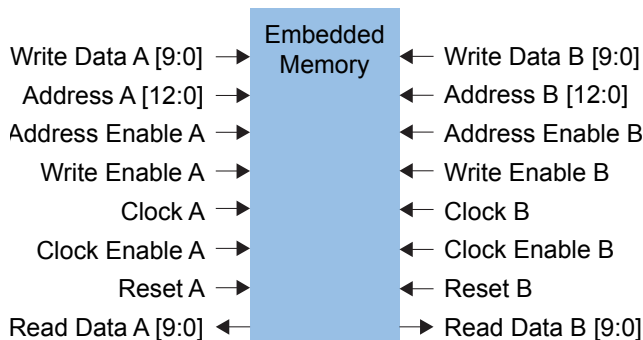
图 3: RAM Block Diagram (True Dual-Port Mode)
