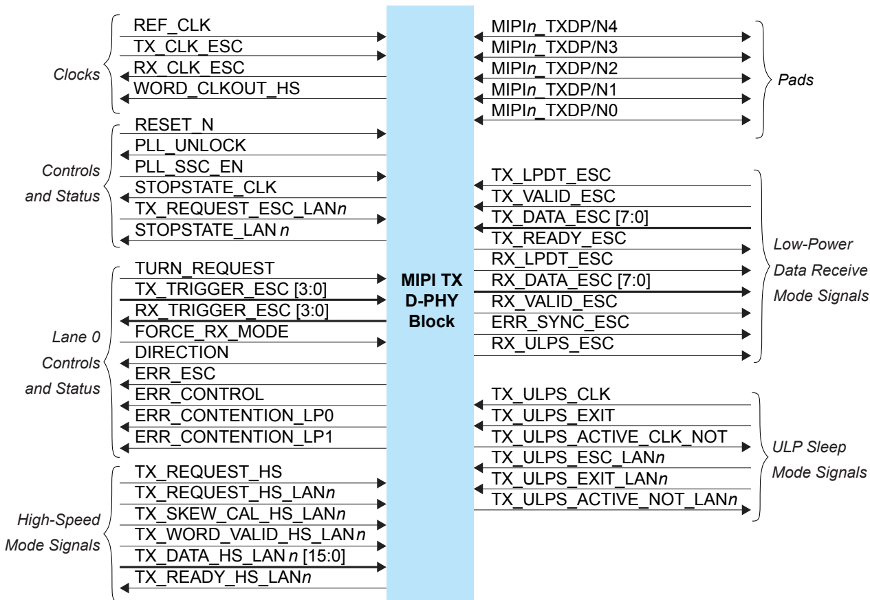
图 36: MIPI TX D-PHY x4 Block Diagram
