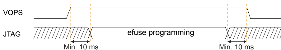
图 45: Fuse Programming Waveform
