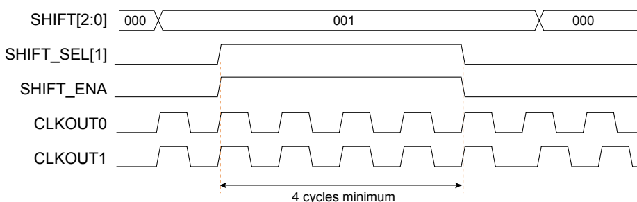
图 40: Single Dynamic Phase Shift Waveform Example for CLKOUT1
