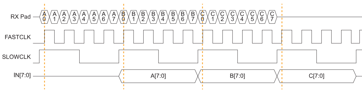
图 25: LVDS RX Timing Example Serialization Width of 8 (Half Rate)
