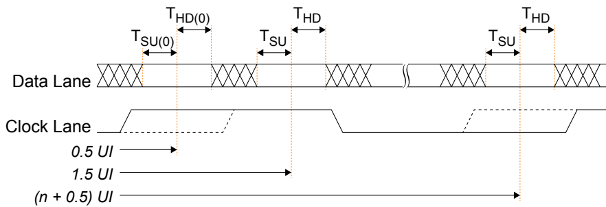
图 31: LVDS RX Timing (Edge-Aligned)
