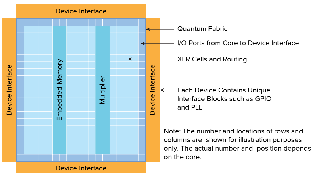
FIG 1: T120 FPGA Block Diagram
