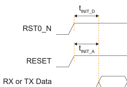
Figure 33: RESET and RST0_N Timing Diagram
