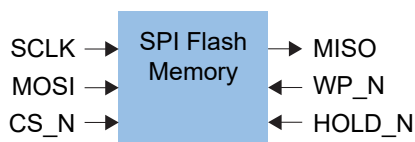
Figure 27: SPI Flash Memory Block Diagram
