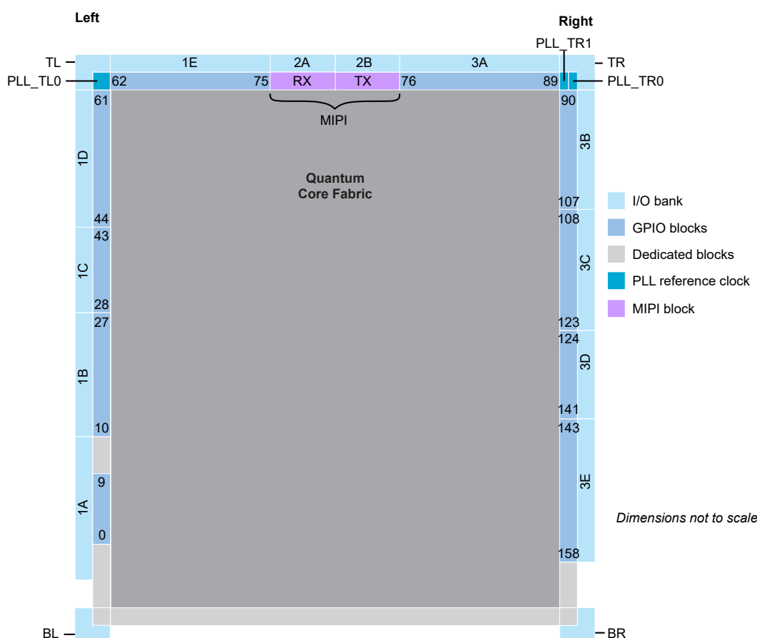
Figure 37: Floorplan Diagram for FPGAs in WLCSP80 Packages (with MIPI)
