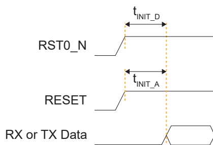
Figure 31: RESET and RST0_N Timing Diagram
