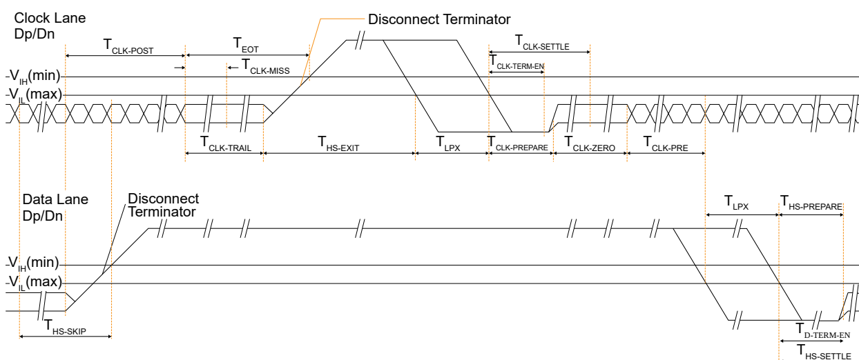
Figure 23: Switching the Clock Lane between Clock Transmission and Low Power Mode Waveform
