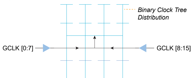
Figure 4: Global Clock Network
