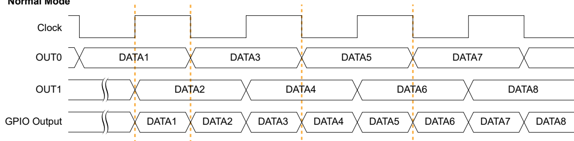
Figure 8: DDIO Output Timing Waveform
