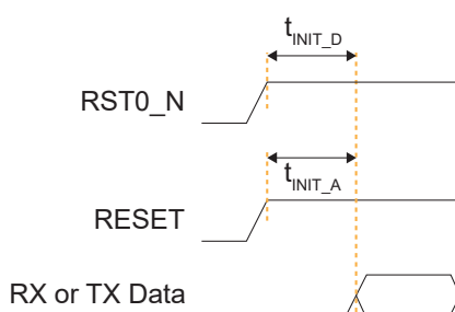
Figure 28: RESET and RST0_N Timing Diagram
