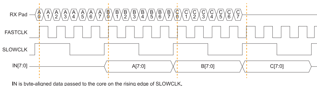
Figure 16: LVDS RX Timing Example Serialization Width of 8
