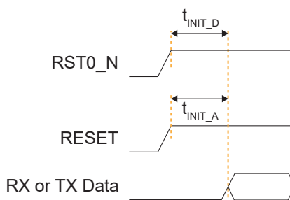
Figure 29: RESET and RST0_N Timing Diagram
