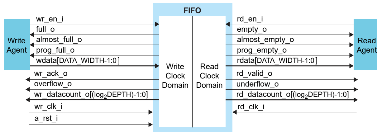
Figure 1: FIFO System Block Diagram
