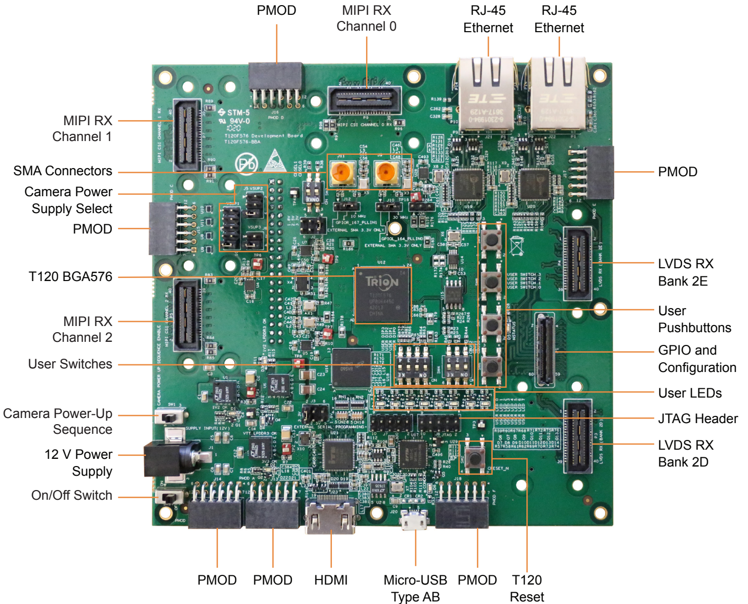
Figure 2 Trion T120 BGA576 Development Kit
