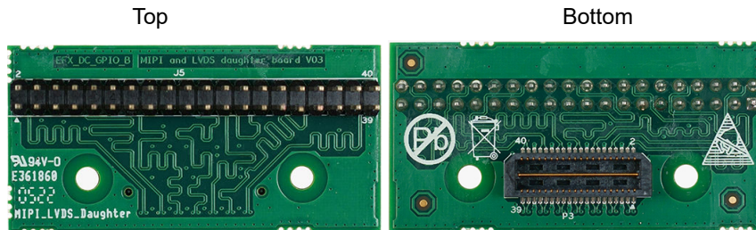
Figure 4: MIPI and LVDS Expansion Daughter Card
