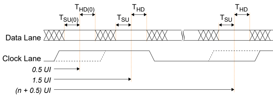
Figure 30: LVDS RX Timing (Edge-Aligned)
