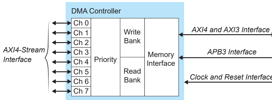
Figure 1: DMA Controller Core Block Diagram
