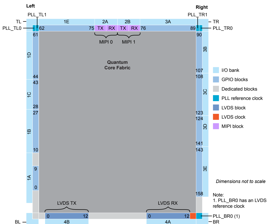
图 39: Floorplan Diagram for FPGAs in BGA169 Packages (with MIPI)
