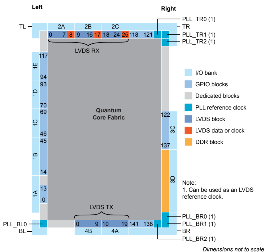
图 42: Floorplan Diagram for FPGAs in BGA400 Packages (with DDR)
