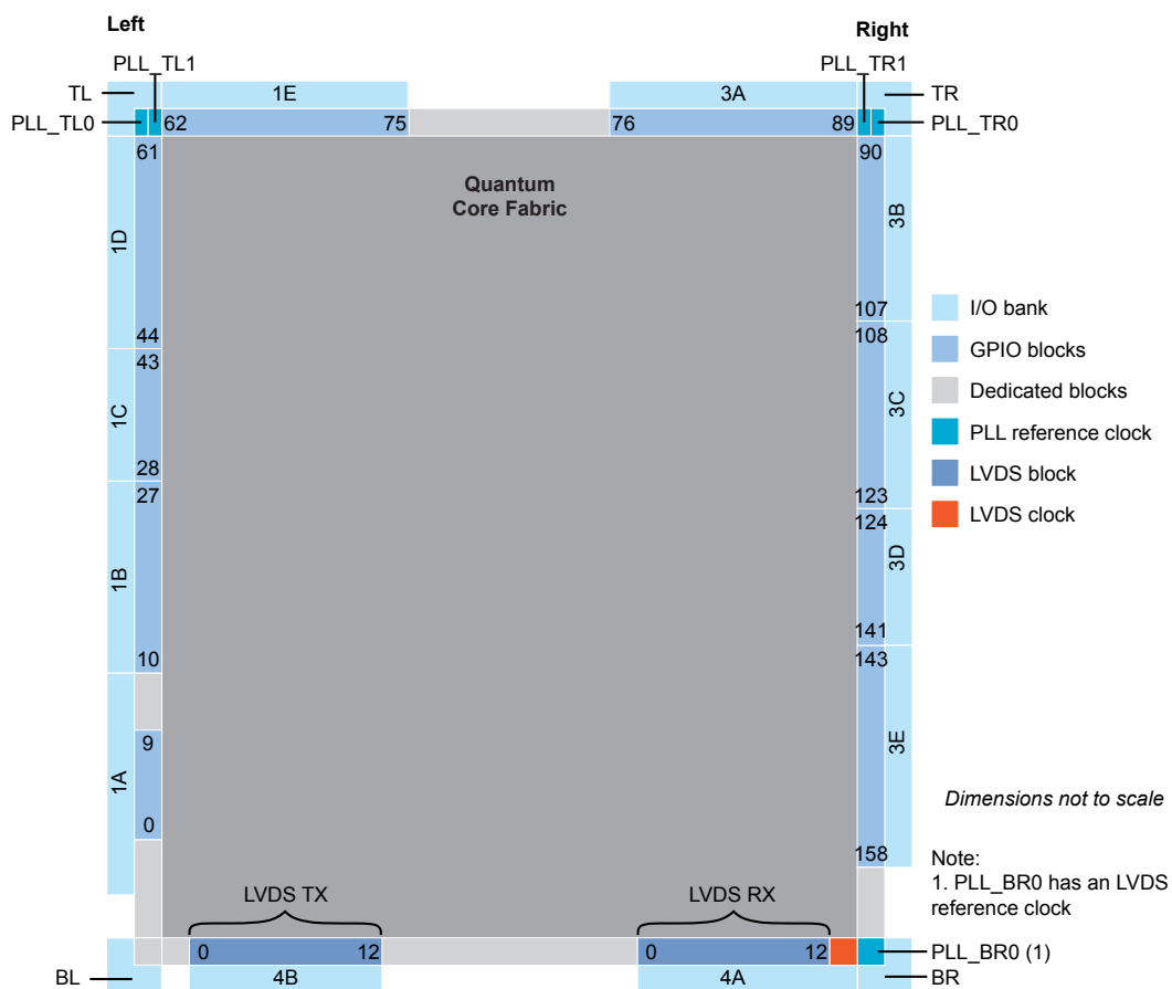
图 38: Floorplan Diagram for QFP100F3 and QFP144 Packages
