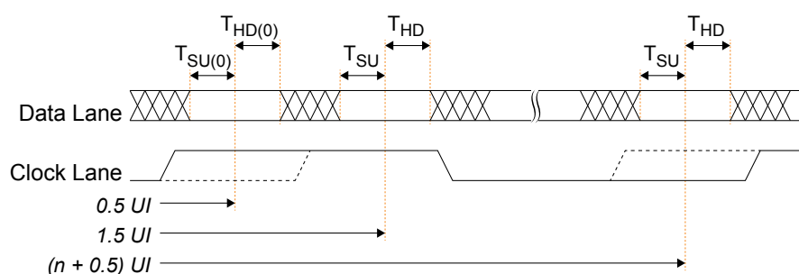
图 32: LVDS RX Timing (Edge-Aligned)
