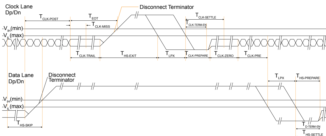
图 24: Switching the Clock Lane between Clock Transmission and Low Power Mode Waveform
