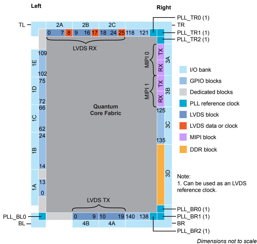
图 36: Floorplan Diagram for BGA324 Packages (with DDR and MIPI)
