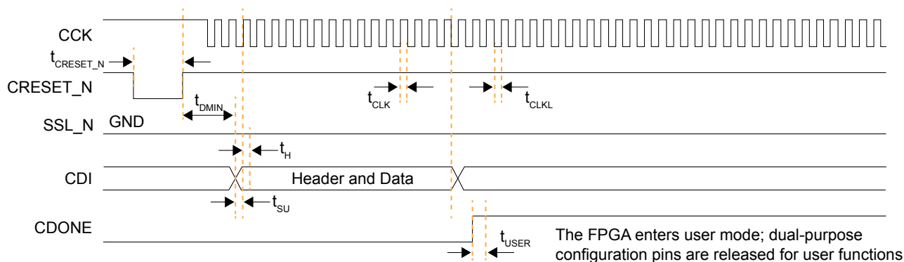
图 34: SPI Passive Mode Timing Sequence
