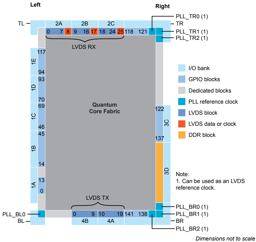
图 37: Floorplan Diagram for BGA400 Packages (with DDR )
