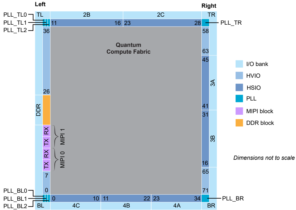
Figure 52: Floorplan Diagram for J361 and M361 Packages
