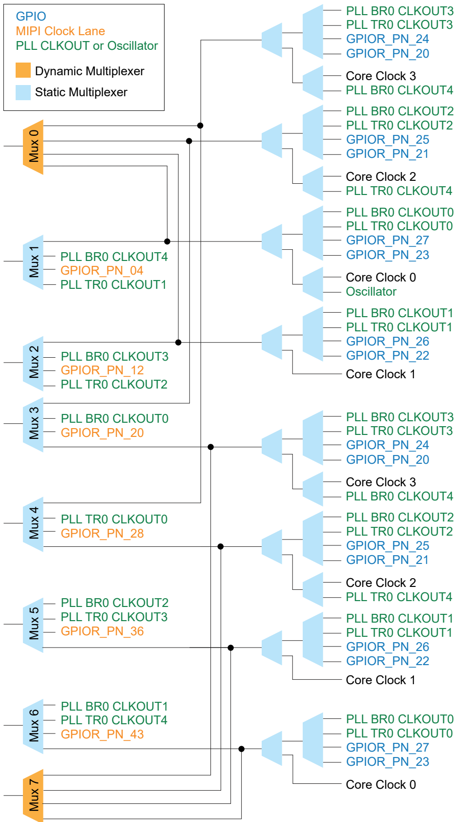
Figure 11: Clock Sources that Drive the Multiplexers: Right
