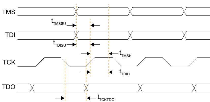
Figure 51: JTAG Timing Waveform
