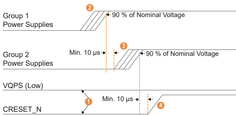
Figure 46: Power-Up Sequence
