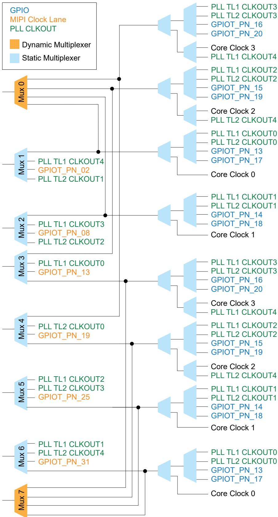
Figure 8: Clock Sources that Drive the Multiplexers: Top
