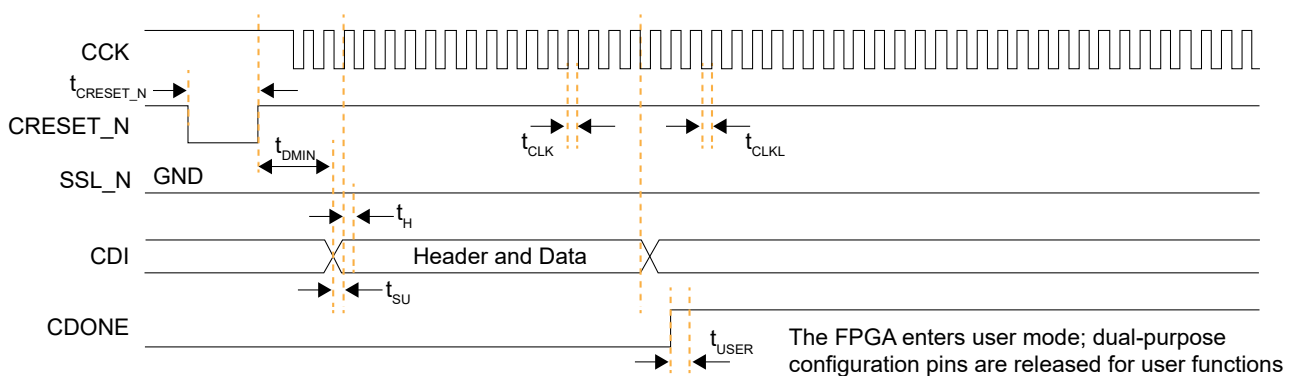
Figure 50: SPI Passive Mode (x1) Timing Sequence
