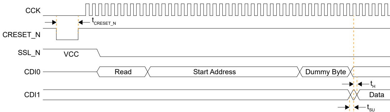
Figure 49: SPI Active Mode (x1) Timing Sequence
