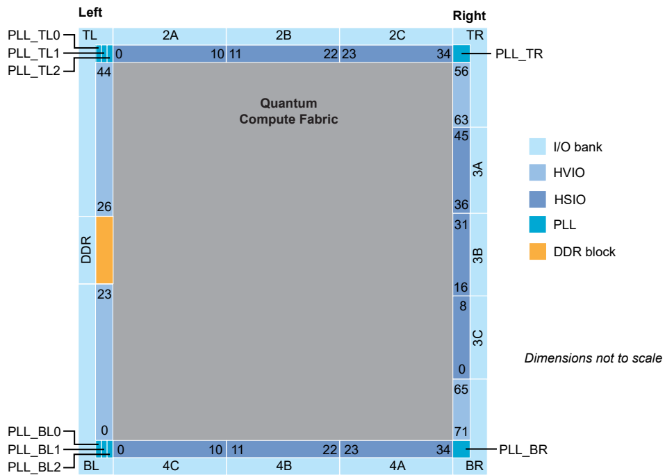
Figure 56: Floorplan Diagram for F529 and G529 Packages
