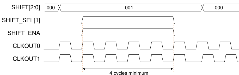
Figure 40: Single Dynamic Phase Shift Waveform Example for CLKOUT1
