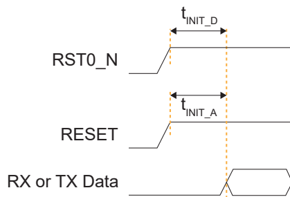
Figure 48: RESET and RST0_N Timing Diagram
