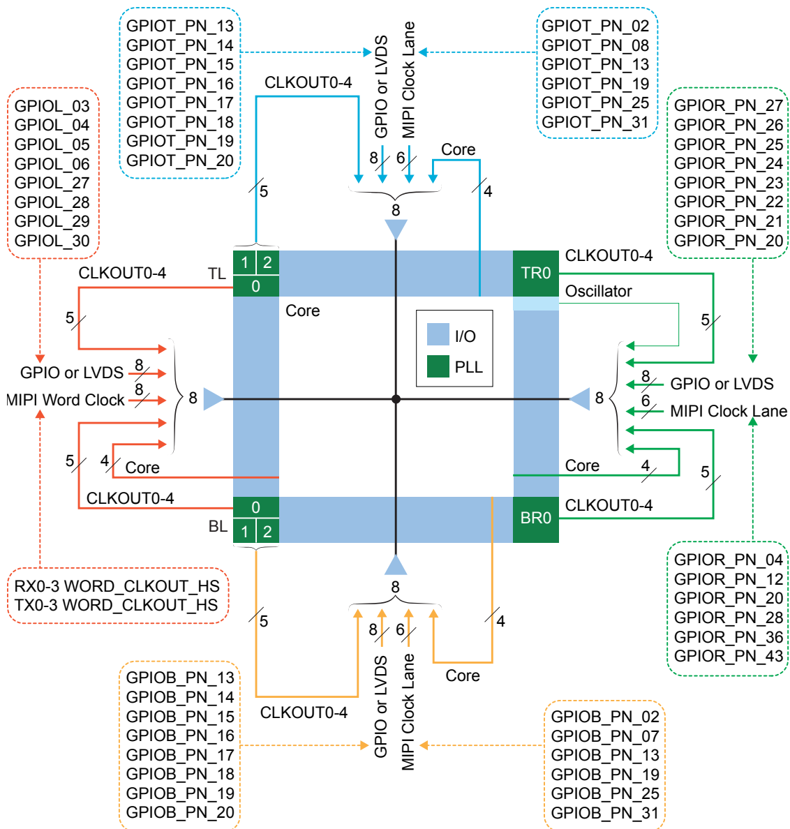
7: Clock Sources that Drive the Global Network
