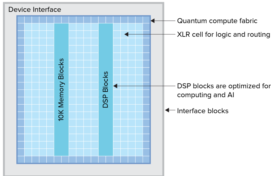
图 1: Ti90 FPGA Block Diagram
