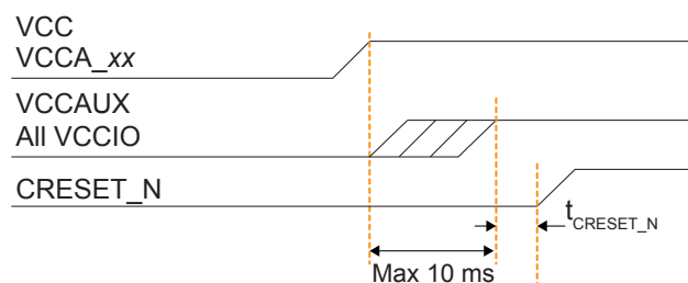
Figure 40: Power-Up Sequence
