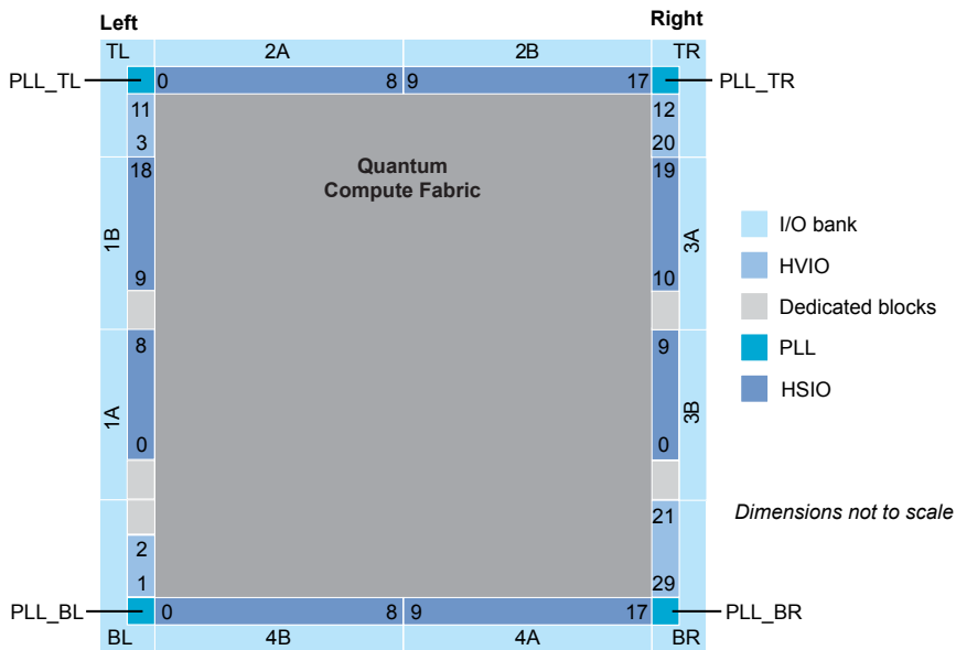
Figure 47: Floorplan Diagram for F225 and F256 Packages
