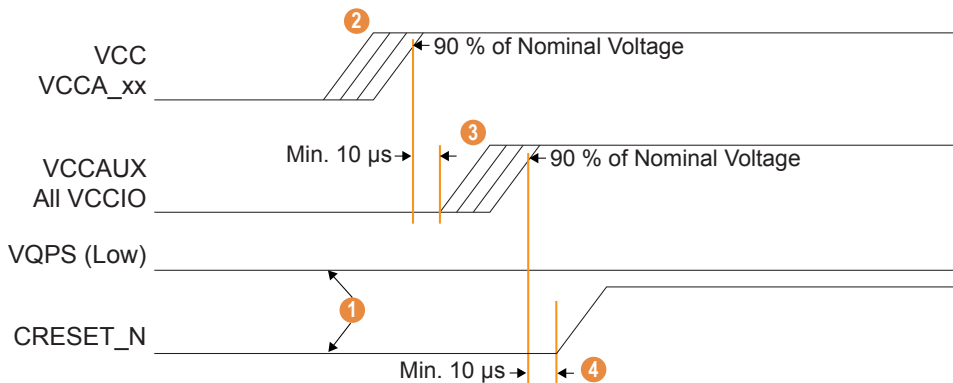
Figure 41: Power-Up Sequence
