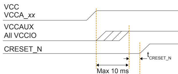
Figure 40: Power-Up Sequence
