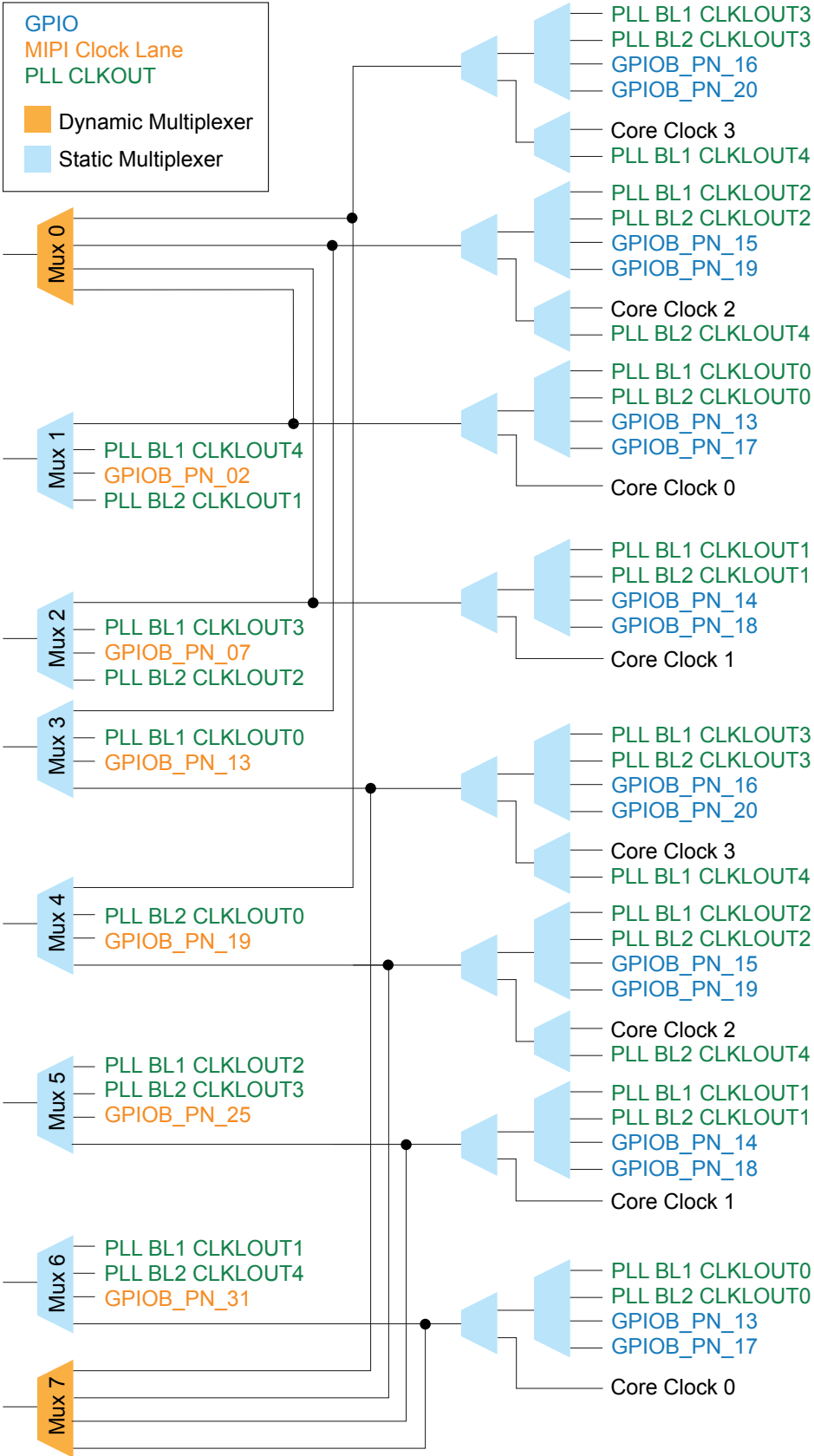
Figure 9: Clock Sources that Drive the Multiplexers: Bottom
