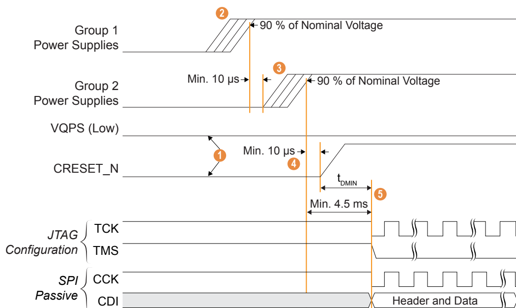
Figure 46: Power-Up Sequence
