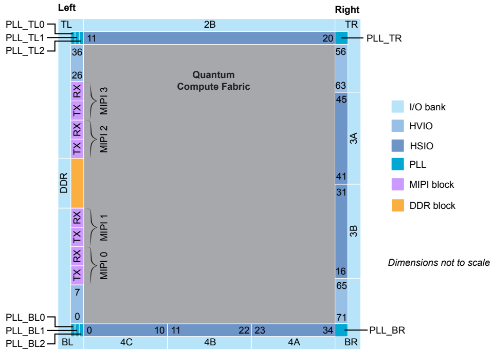
Figure 55: Floorplan Diagram for J484 Packages
