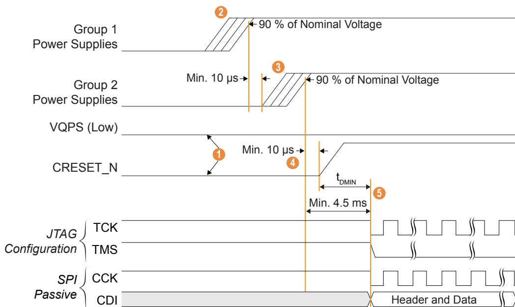
Figure 46: Power-Up Sequence
