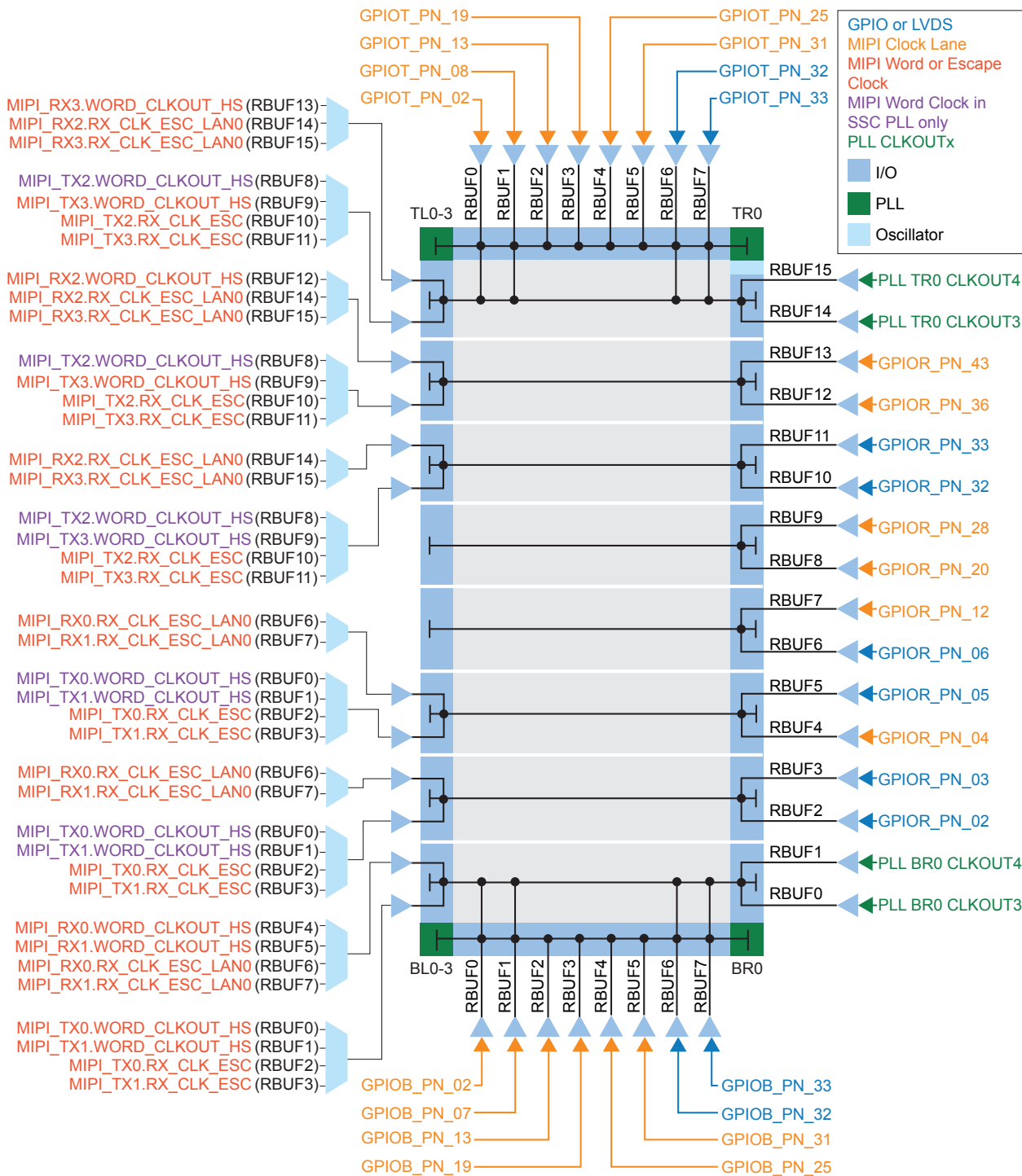
Figure 12: Clock Sources that Drive the Regional Network
