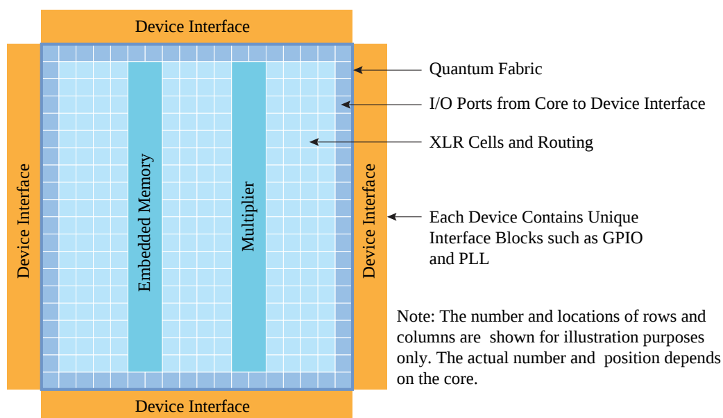
Figure 1: T85 FPGA Block Diagram
