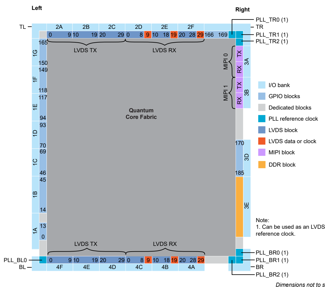
Figure 36: Floorplan Diagram for F324 Packages (with DDR and MIPI)
